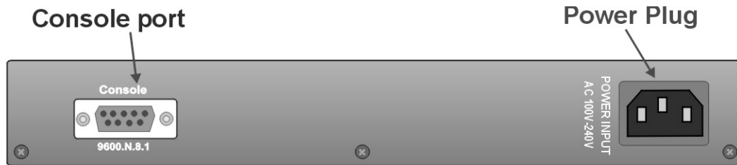
Figure 2-5. The Rear Panel of the switch
